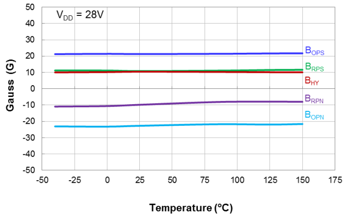
Switch Points B_{OP} and B_{RP} vs Temperature
