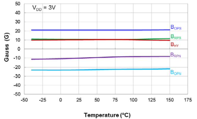
Switch Points B_{OP} and B_{RP} vs Temperature
