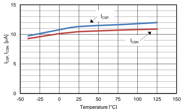
Figure 10. I_{CSP} , I_{CSN} vs Temperature
