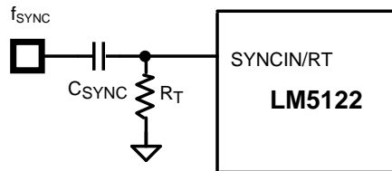
Figure 25. Oscillator Synchronization Through AC Coupling in Master1 Mode
