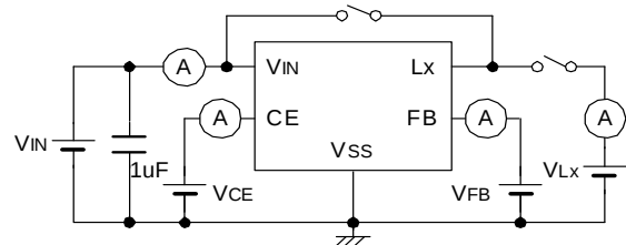
●Circuit ③
