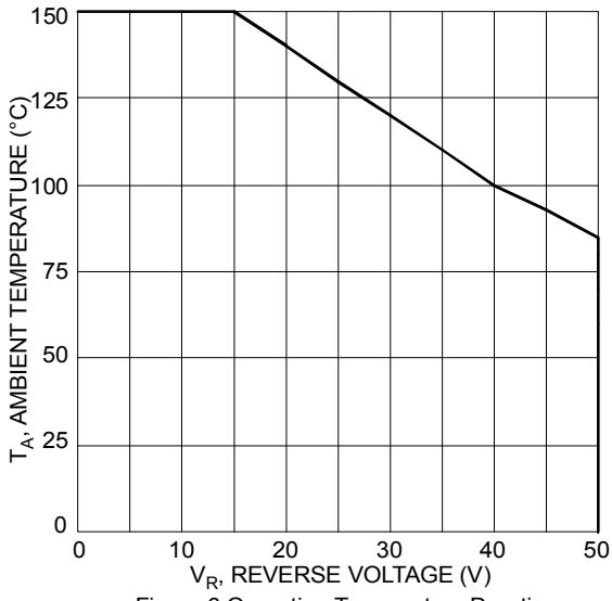
Figure 6 Operating Temperature Derating
