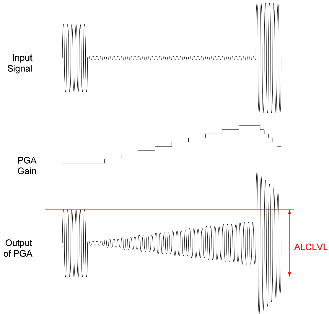
Figure 14 ALCLVL
