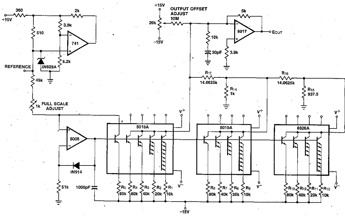
Figure 7: PNP Reference
