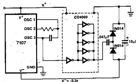
Figure 10: Generating Negative Supply from +5v
