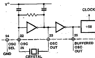
Figure 11: Crystal Oscillator
