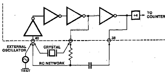
Figure 8: Clock Circuits
