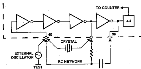
Figure 7. Clock Circuits
