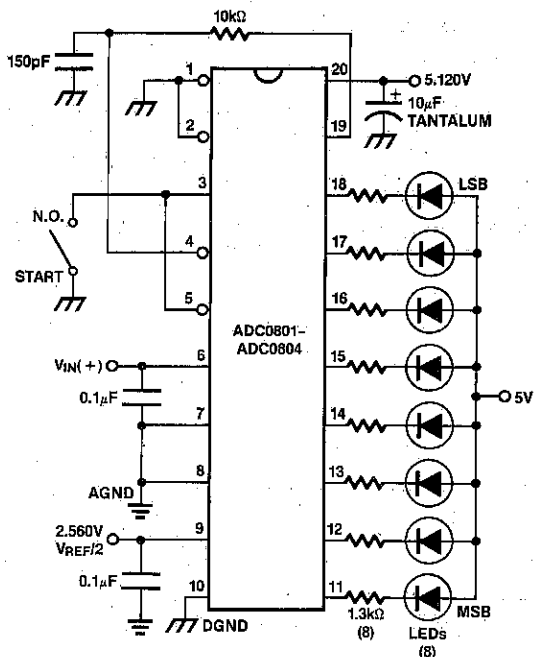
Figure 9. Basic Tester for the A/D
