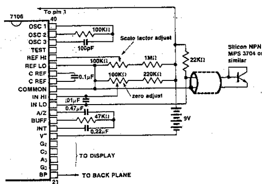
Figure 18: 7106 used as a digital centigrade thermometer. A silicon diode-connected transistor has a temperature coefficient of about -2\text{mV}/^\circ\text{C} . Calibration is achieved by placing the sensing transistor in ice water and adjusting the zeroing potentiometer for a 000.0 reading. The sensor should then be placed in boiling water and the scale-factor potentiometer adjusted for 100.0 reading.
