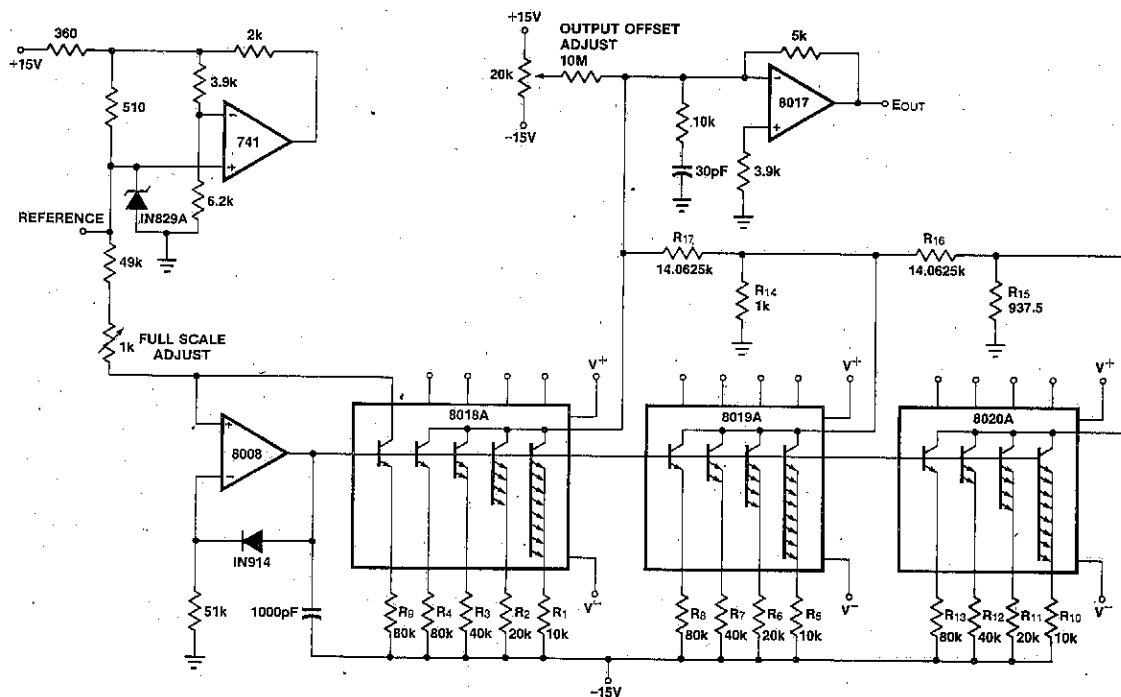
Figure 7: PNP Reference
