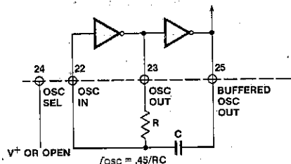
Figure 10: RC Oscillator
