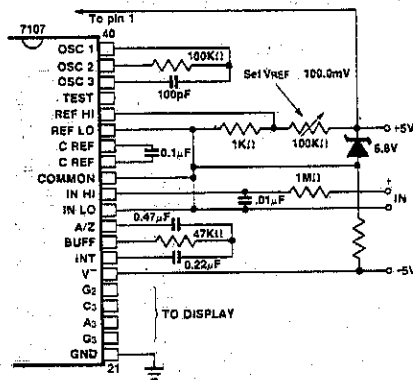
Figure 14: 7107 with Zener diode reference. Since low T.C. zeners have breakdown voltages ~ 6.8V, diode must be placed across the total supply (10V). As in the case of Figure 12; 1N LO. may be tied to either COMMON or GND.
