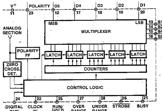
Figure 5: Digital Section 7135
