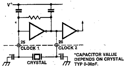
Figure 11: Crystal Oscillator
