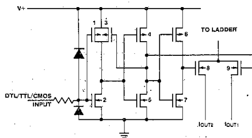
Figure 8. CMOS Switch
