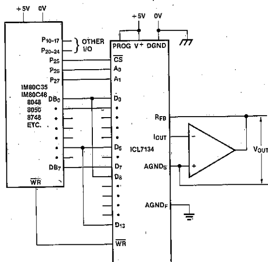
Figure 11. ICL7134 Interface to MCS-48 System.
