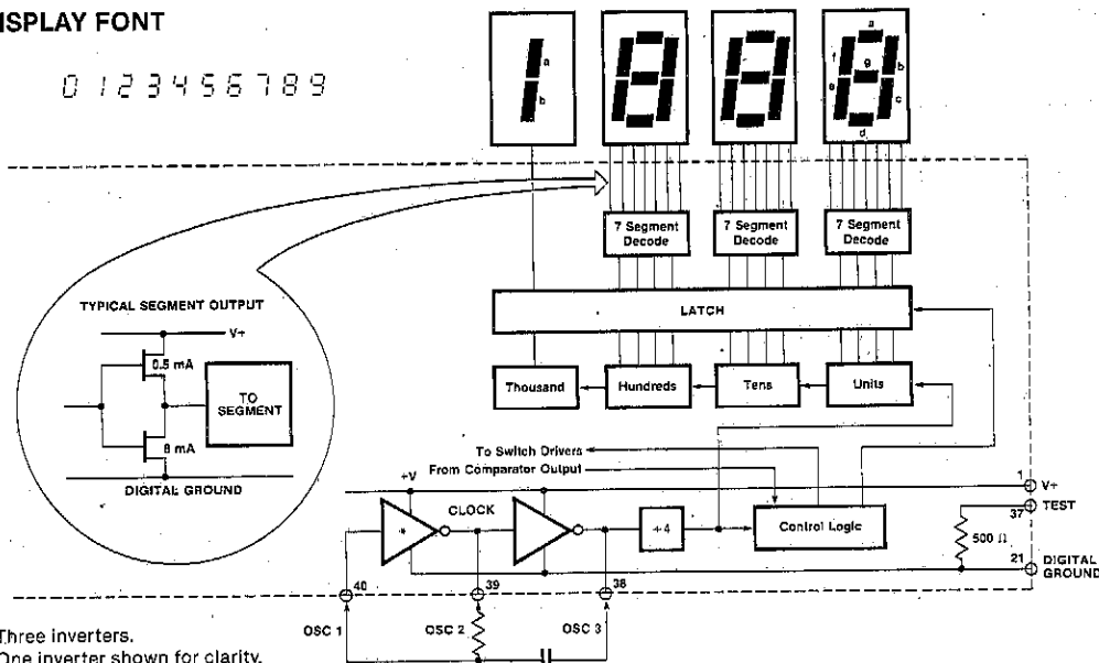
Figure 5. Digital Section
