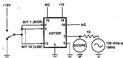
Figure 4. Output Capacitance
