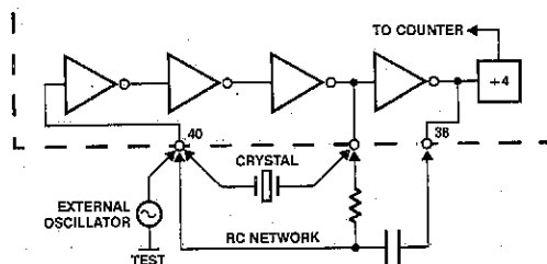
Figure 7. Clock Circuits
