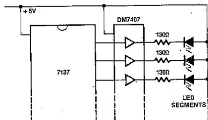
Figure 6. Display Buffering for Increased Drive Current.
