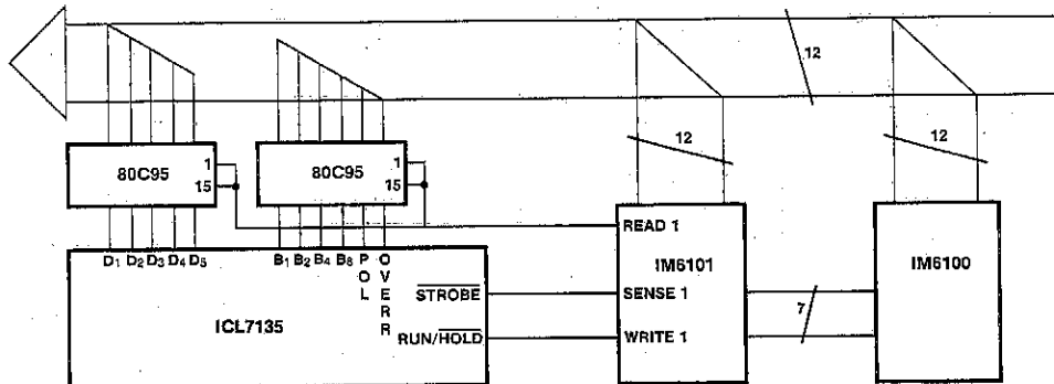
Figure 15: Complex ICL7135 to UART Interface
