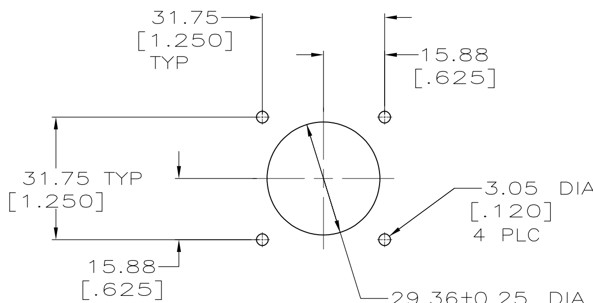
FRONT MOUNTED PANEL CUTOUT SCALE 1:1
