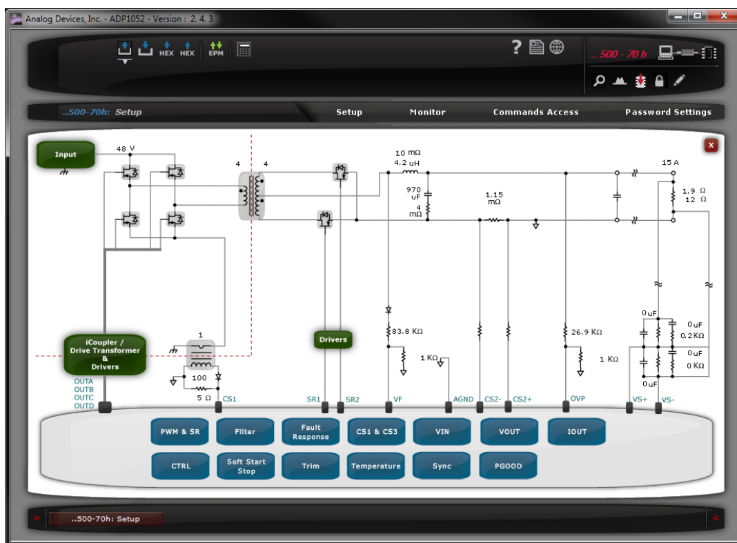
Figure 61. GUI Software
