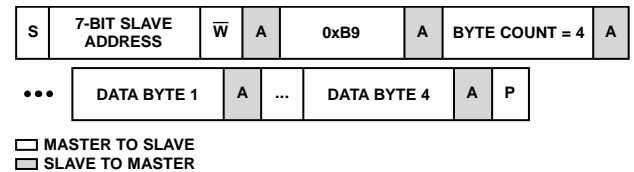
Figure 60. Write Four Bytes to Page 9
