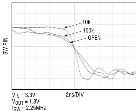
Figure 5. Slew Rate at SW Pin vs SRLIM/DDR Resistor: Open, 100k, 10k
