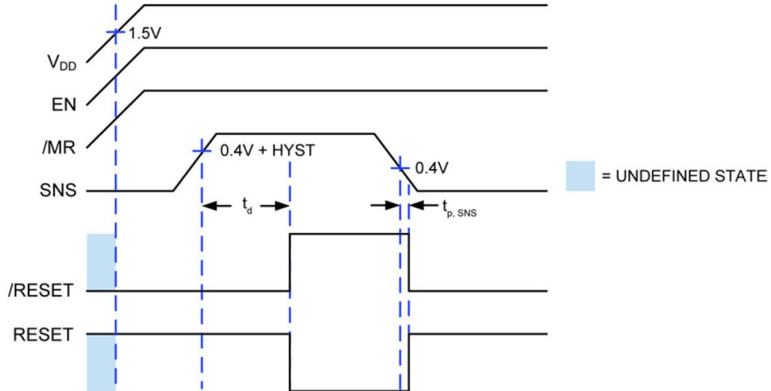
Figure 1. Timeout and Propagation Delay from Sense to RESET and /RESET
