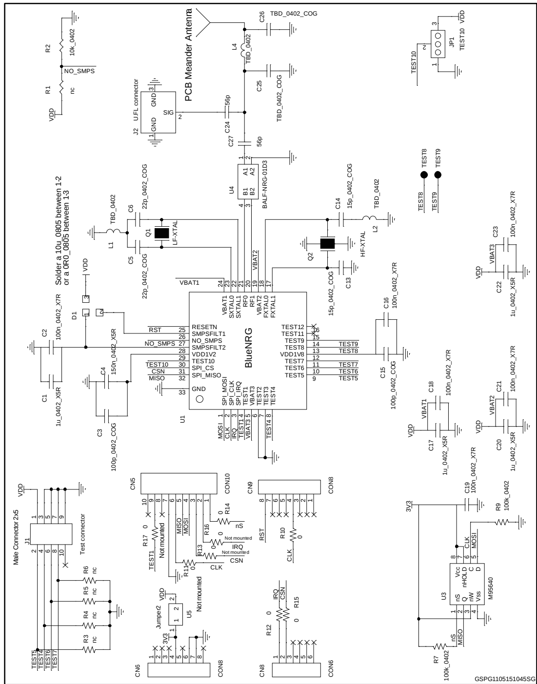
Figure 2: Circuit schematic
