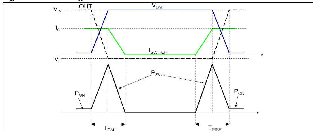
Figure 14. Switching losses
