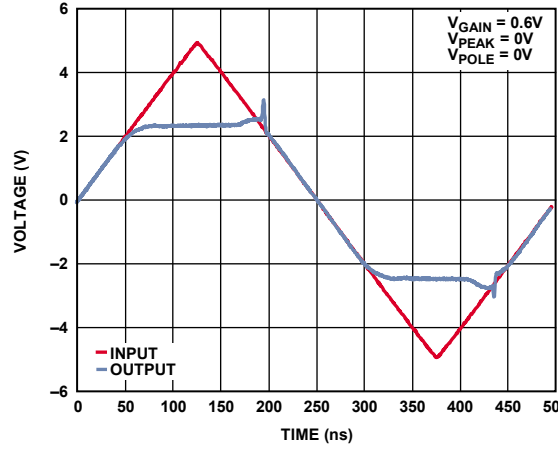
Figure 10. Overdrive Recovery
