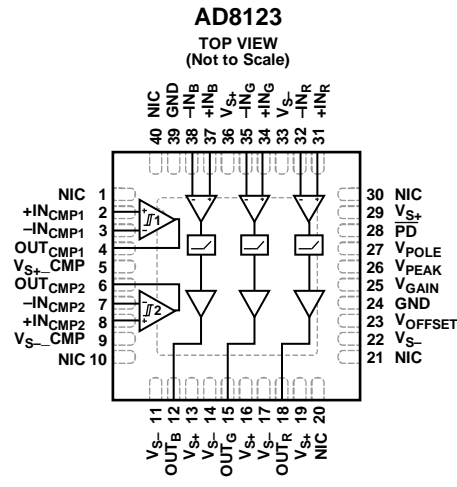
Figure 4. Pin Configuration
