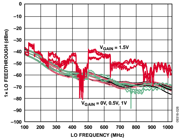
Figure 46. 1x LO Feedthrough vs. LO Frequency, V_{GAIN} Supply, and Temperature (Narrow-Band Mode)
