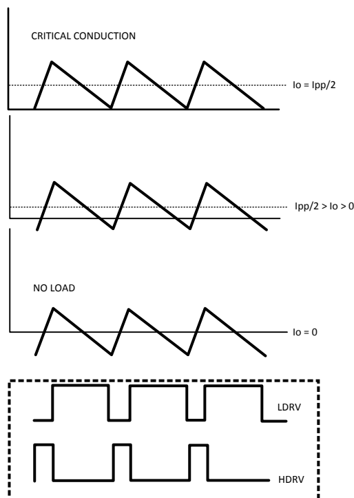
Figure 10. Inductor Current in FPWM Mode
