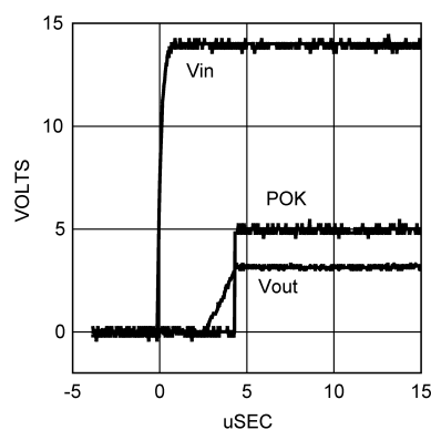
Figure 13. Startup Power OK
