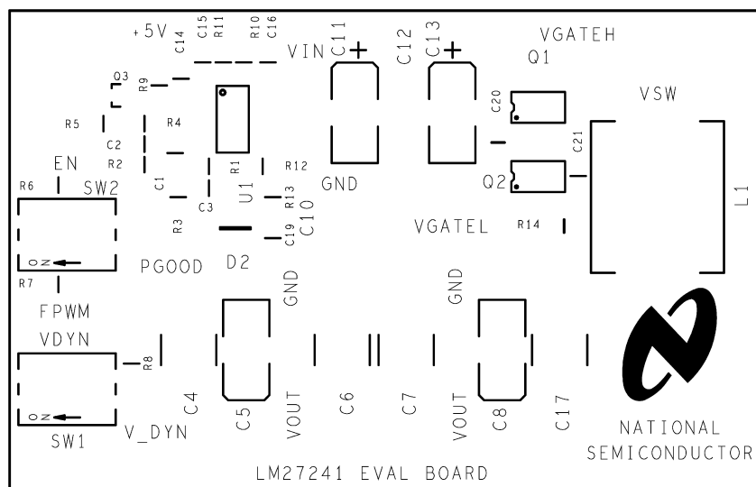
Figure 24. Top Overlay
