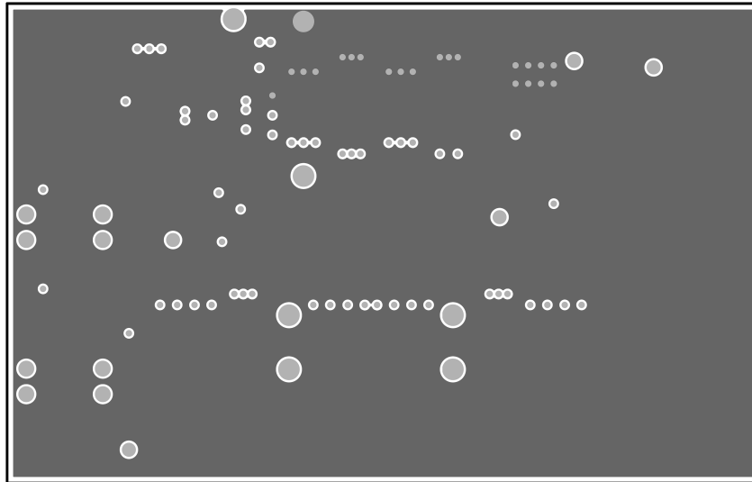
Figure 27. Internal Plane 2
