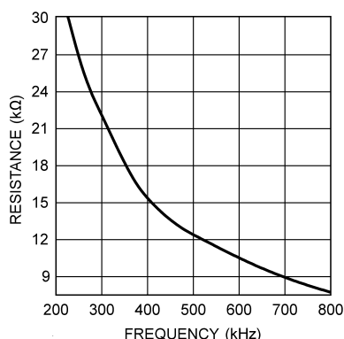
Figure 20. Frequency Adjust Resistor Guideline
