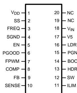
Figure 2. Top View 20-Lead TSSOP (PW)
