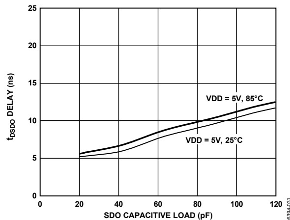
Figure 23. t_{\text{DSDO}} Delay vs. Capacitance Load and Supply
