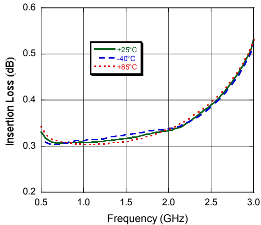
Insertion Loss
