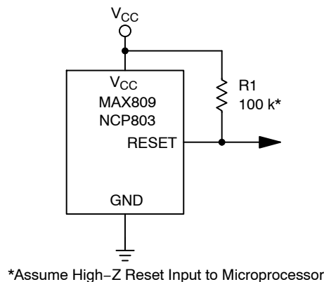
Figure 14. RESET Signal Integrity
