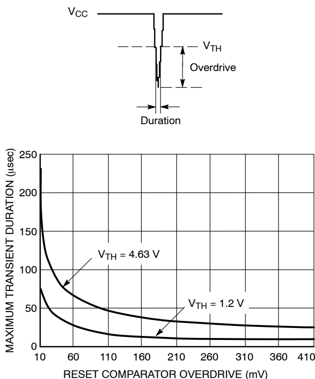
Figure 13. Maximum Transient Duration vs. Overdrive for Glitch Rejection at 25°C
