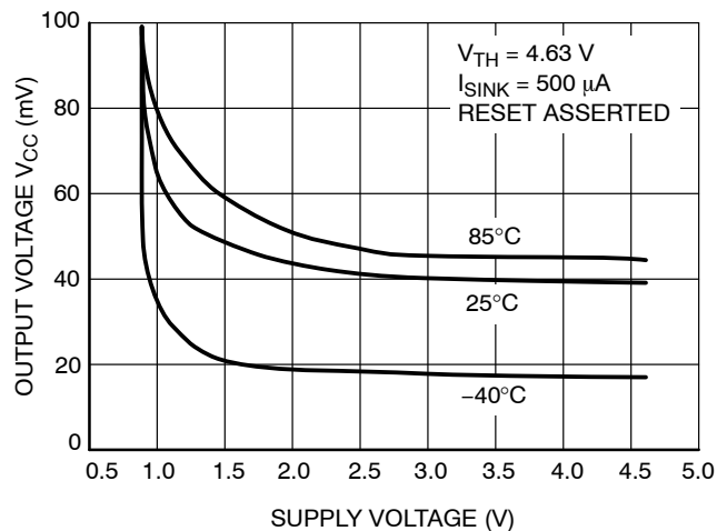
Figure 8. Output Voltage Low vs. Supply Voltage
