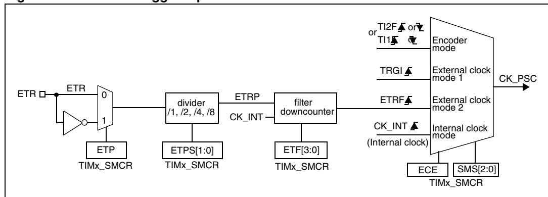
Figure 29. External trigger input block
