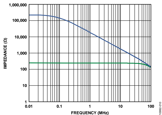
Figure 10. R_{IN} vs. Frequency
