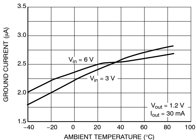
Figure 6. Ground Pin Current vs. Temperature
