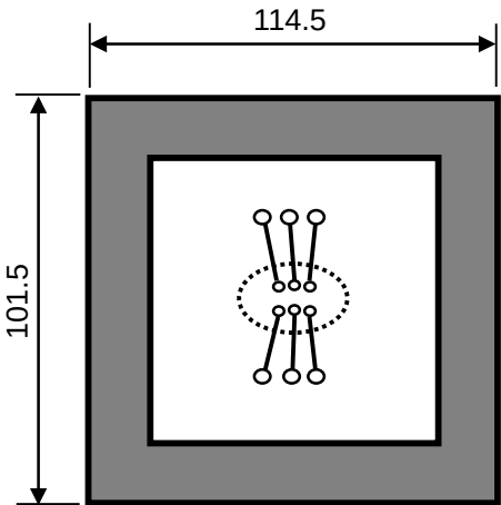
IC Mount Area (mm) Measurement Board Pattern
