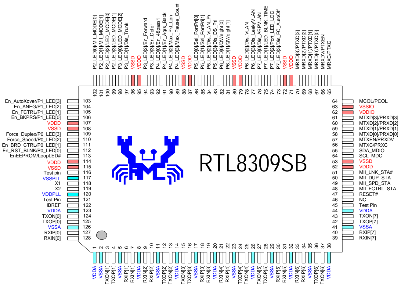
Figure 2. Pin Assignments
