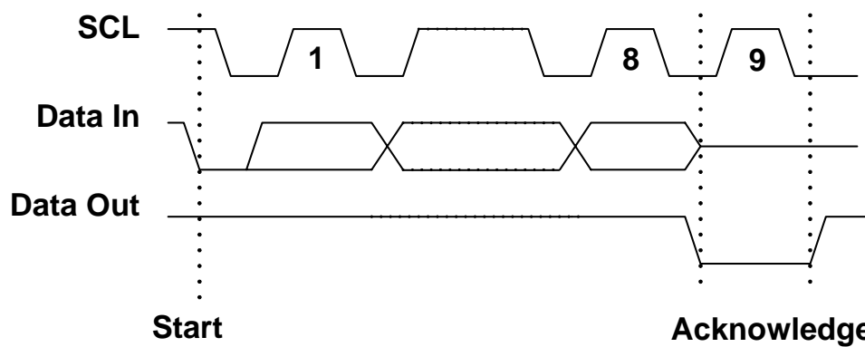
Figure 11. Output Acknowledge
