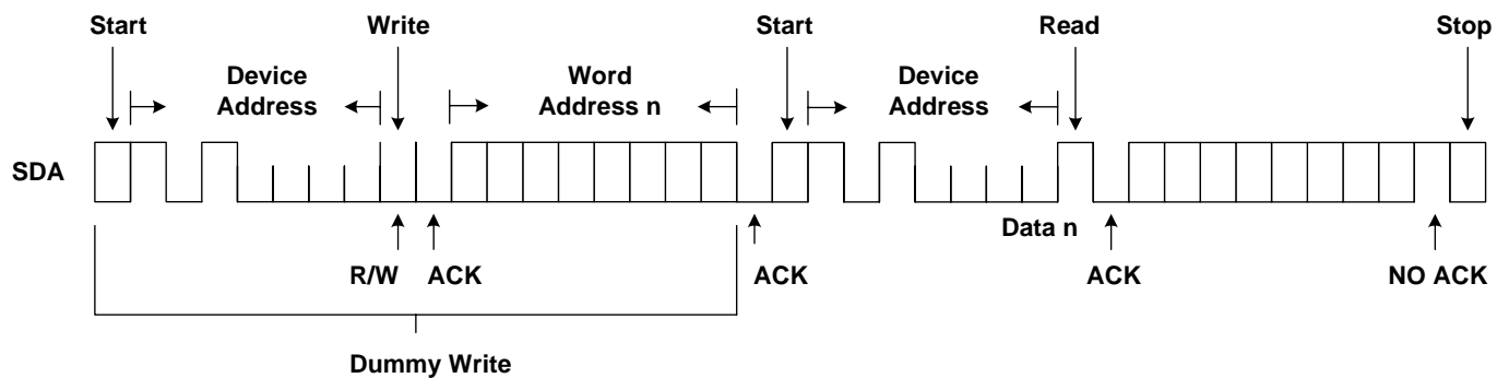
Figure 12. Random Read
