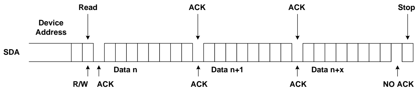
Figure 13. Sequential Read
