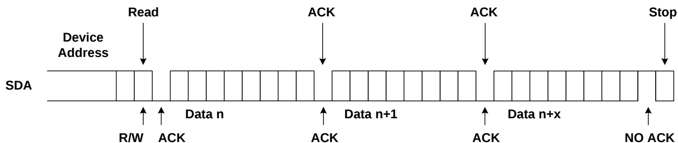
Figure 13. Sequential Read
