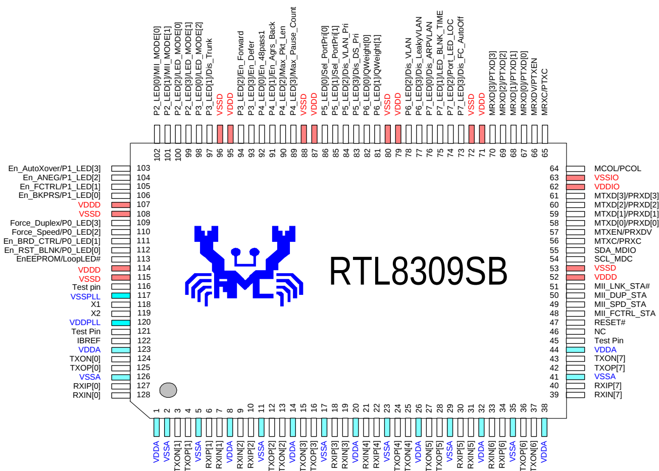
Figure 2. Pin Assignments
