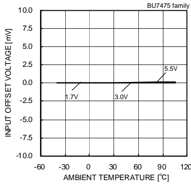
Fig.152 Input Offset Voltage – Ambient Temperature (Vicm=VDD-1.2[V], VOVT=1.5[V])
