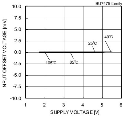
Fig.151 Input Offset Voltage – Supply Voltage (Vicm=VDD-1.2[V], VOVT=1.5[V])
