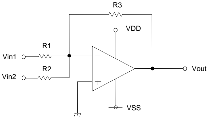
Fig.170 Adder circuit
