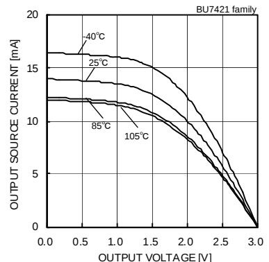
Fig.124 Output Source Current - Output Voltage (VDD=3[V])
