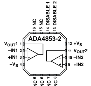
Figure 2. 16-Lead LFCSP_VQ
