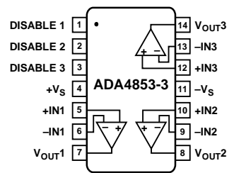
Figure 4. 14-Lead TSSOP
