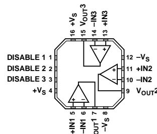
Figure 3. 16-Lead LFCSP_VQ ADA4853-3
