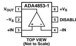
Figure 1. 6-Lead SC70 ADA4853-1
