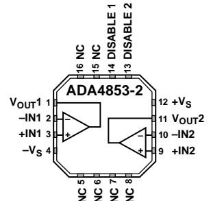
Figure 2. 16-Lead LFCSP_VQ ADA4853-2
