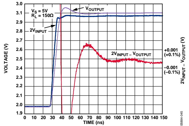
Figure 46. 0.1% Settling Time
