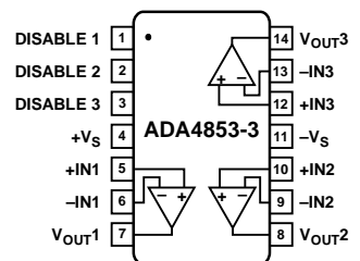
Figure 4. 14-Lead TSSOP ADA4853-3
