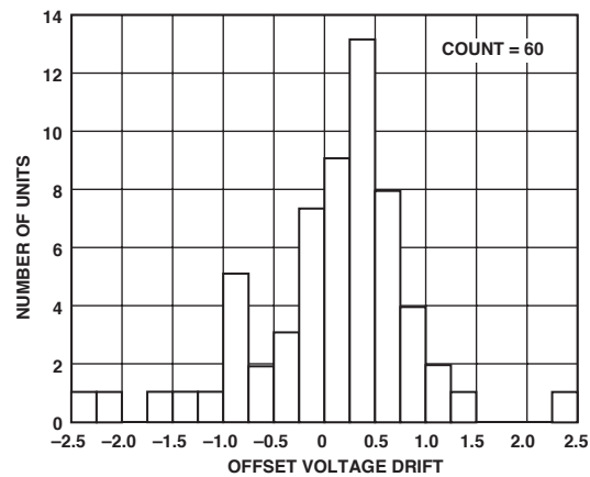
TPC 13. TC V_{OS} Distribution, -55^{\circ}\text{C} to +125^{\circ}\text{C} , V_S = 5, 0
