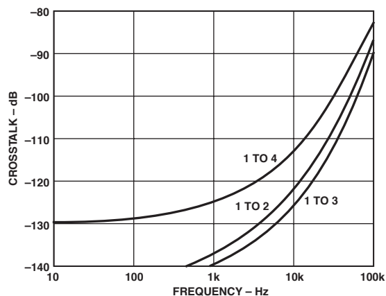
TPC 22. Crosstalk vs. Frequency
