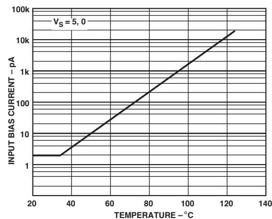
TPC 15. Input Bias Current vs. Temperature
