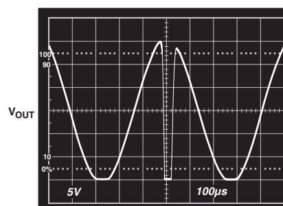
TPC 8. Phase Reversal with Inputs Exceeding Supply by 1 V
