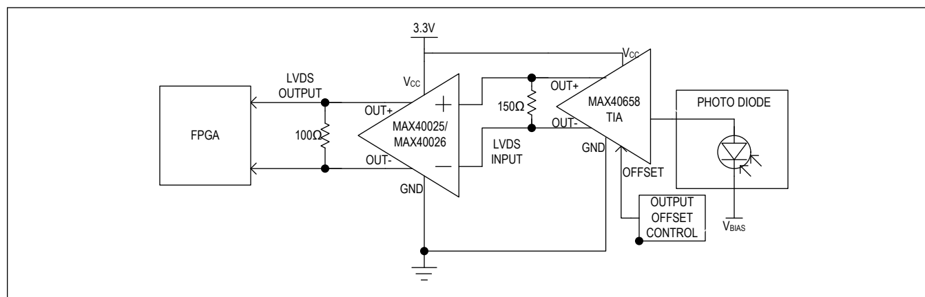
Receiver Section of Single-Ended Time-of-Flight Measurement Circuit:
