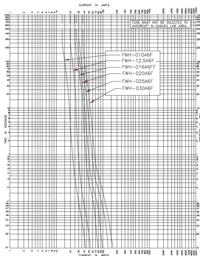
Time-Current Curve
