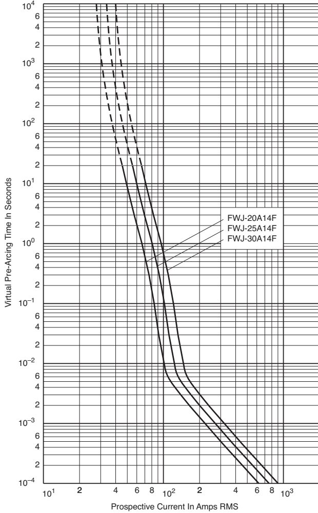
Time-Current Curve
