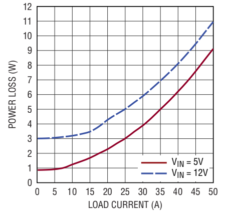
Figure 16. 3.3V OUT Power Loss Curve
