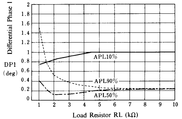
Differential Phase 1 vs. Load Resistor
