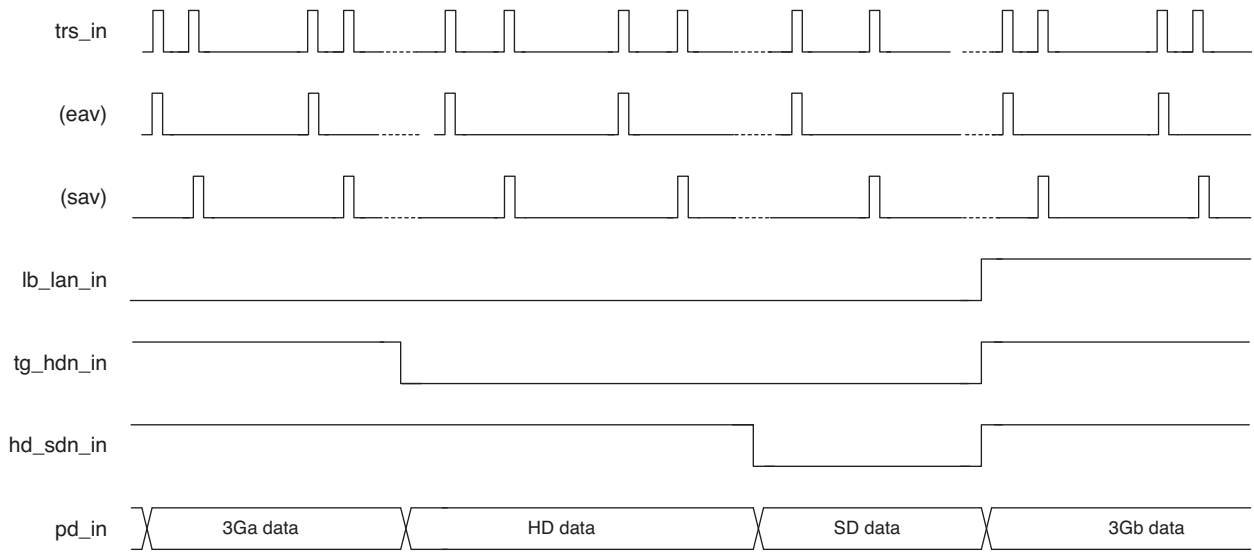
Figure 2-12. Rate-select Control Signals for Different Transmit Rates
