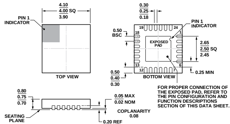
Figure 40. 24-Lead Lead Frame Chip Scale Package [LFCSP_WQ] 4 mm × 4 mm Body, Very Very Thin Quad (CP-24-7)
