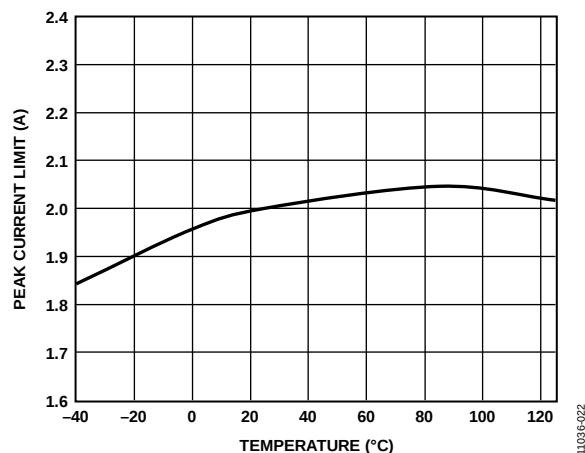
Figure 22. Peak Current Limit Threshold vs. Temperature
