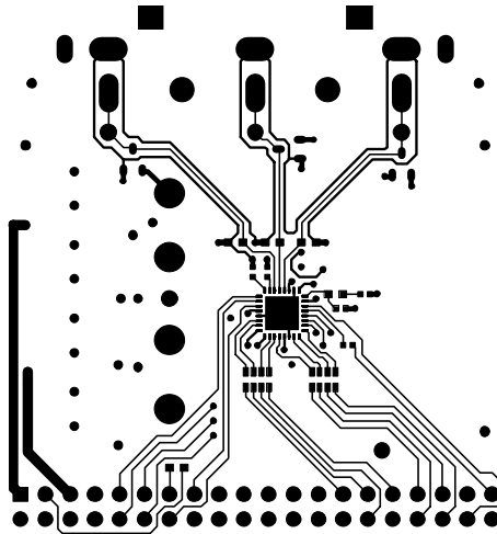
Figure 18: EVAL-ADV7390/91EBZ Component Side Layer 1
