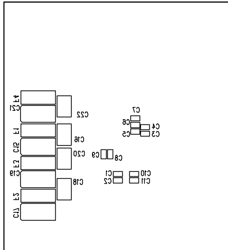
Figure 30: EVAL-ADV7392/93EBZ Silkscreen Bottom
