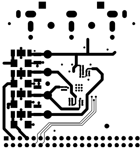
Figure 29: EVAL-ADV7392/93EBZ Layer 4
