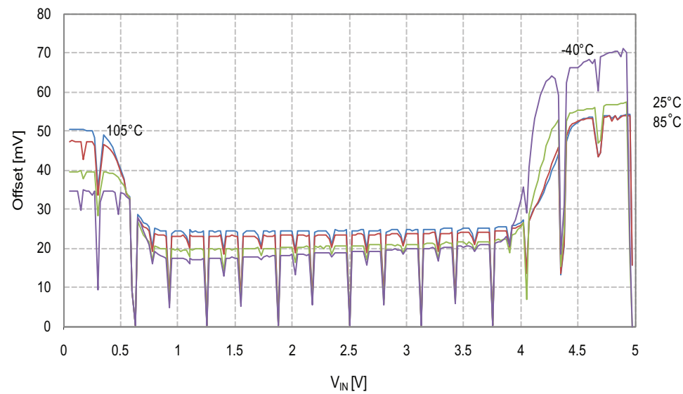
Figure 26-58. Analog Comparator Offset vs. V_{IN} ( V_{CC} = 5V )
