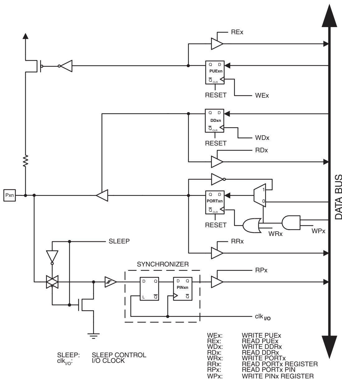
Figure 10-2. General Digital I/O (1)
