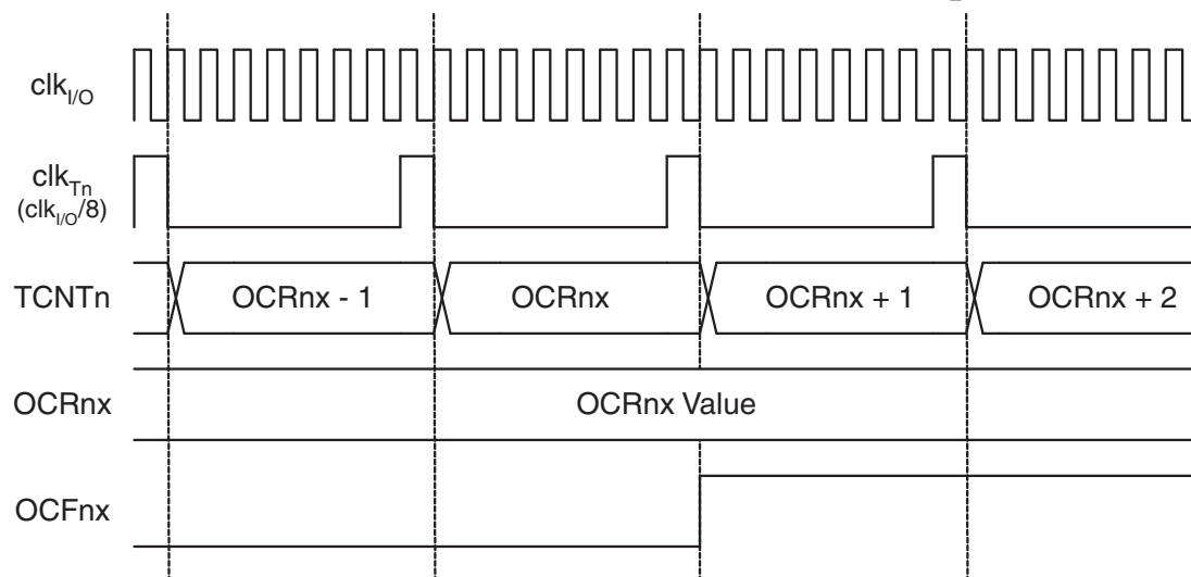
Figure 12-11. Timer/Counter Timing Diagram, Setting of OCF1x, with Prescaler ( f_{\text{clk}_{I/O}}/8 )
