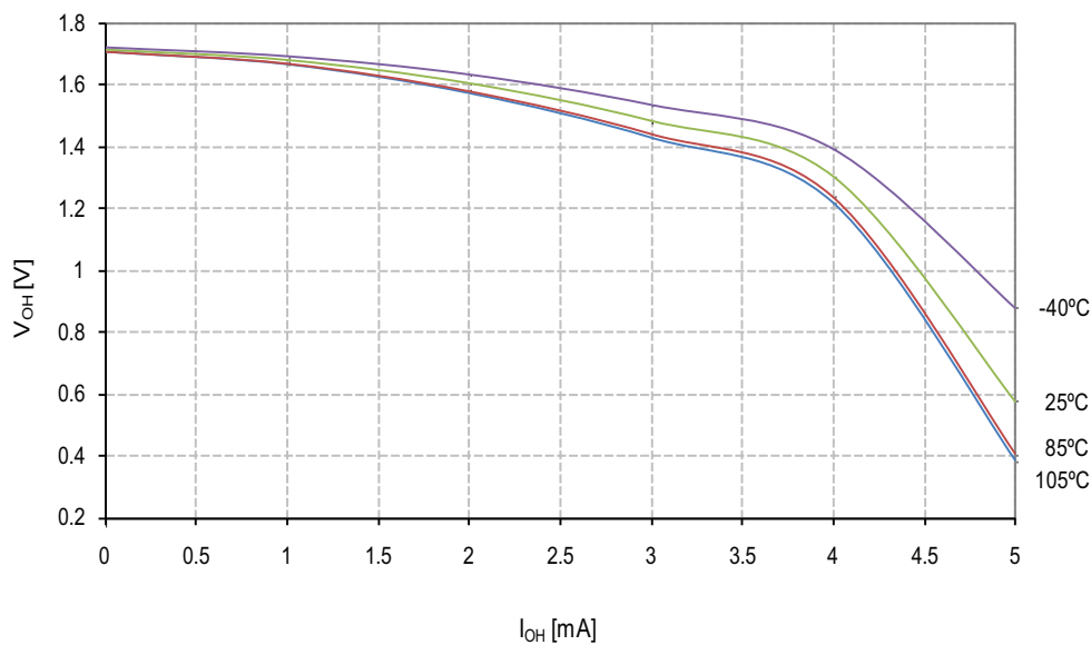
Figure 26-34. V_{OH} : Output Voltage vs. Source Current (I/O Pin, V_{CC} = 1.8V )
