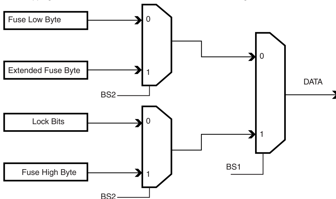
Figure 23-6. Mapping Between BS1, BS2 and the Fuse and Lock Bits During Read
