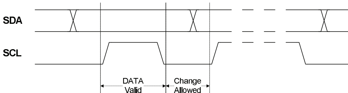
Figure 14-4. Data Validity
