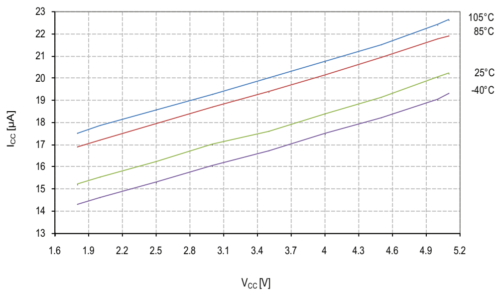
Figure 26-19. Brownout Detector Current vs. V_{CC}
