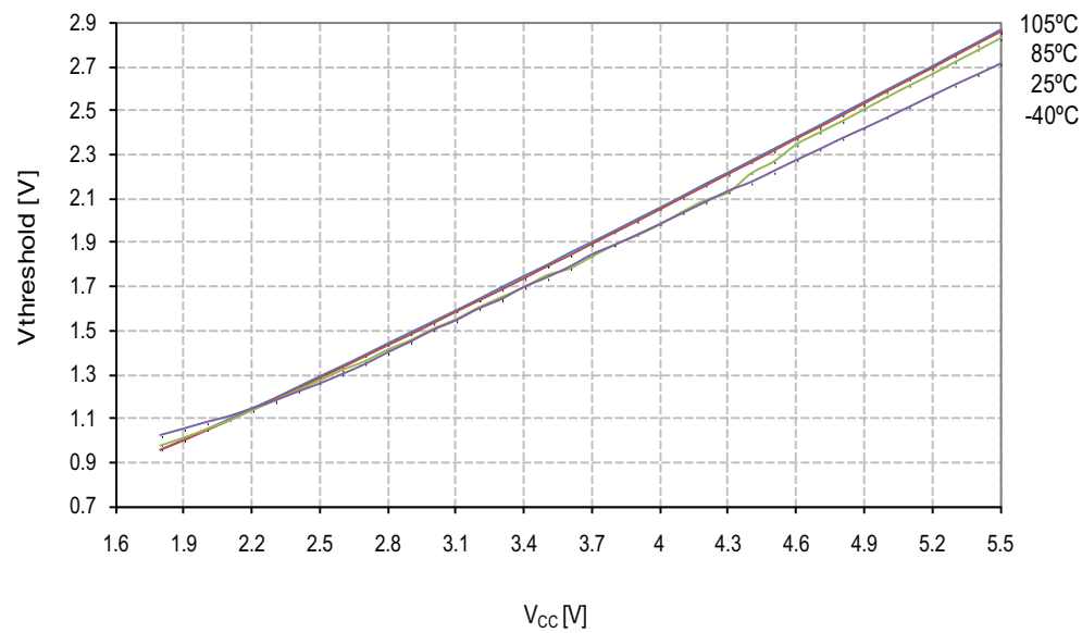
Figure 26-28. V_{IH} : Input Threshold Voltage vs. V_{CC} (I/O Pin, Read as '1')
