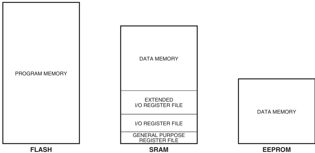
Figure 5-1. Memory Overview.
