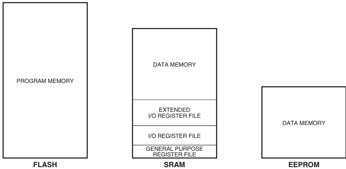
Figure 5-1. Memory Overview.
