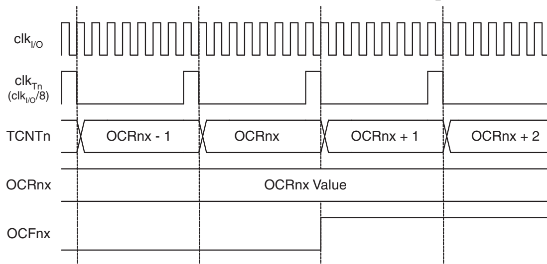
Figure 12-11. Timer/Counter Timing Diagram, Setting of OCF1x, with Prescaler ( f_{\text{clk\_I/O}}/8 )
