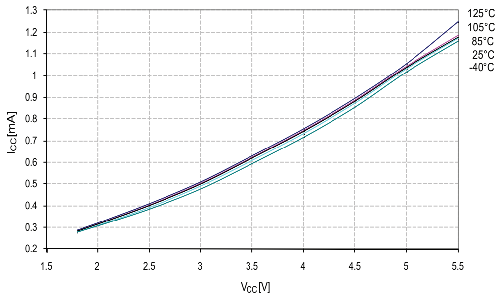
Figure 26-4. Active Supply Current vs. V_{CC} (Internal Oscillator, 1 MHz)
