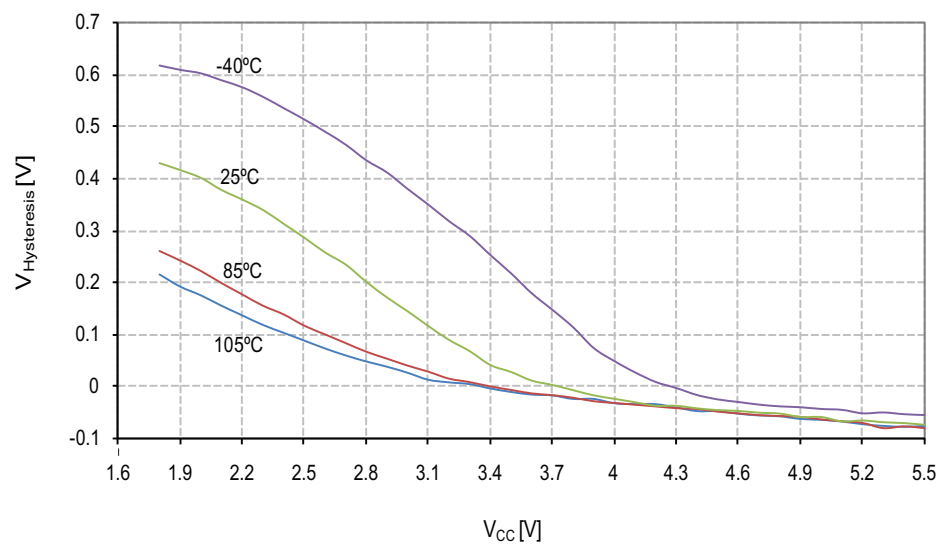
Figure 26-56. V_{IH}-V_{IL} : Input Hysteresis vs. V_{CC} (Reset Pin )
