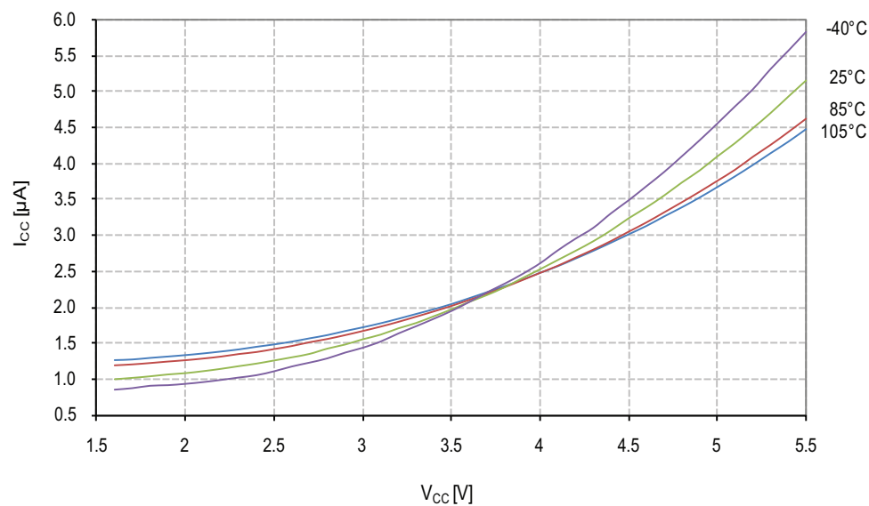
Figure 26-18. Watchdog Timer Current vs. V_{CC}
