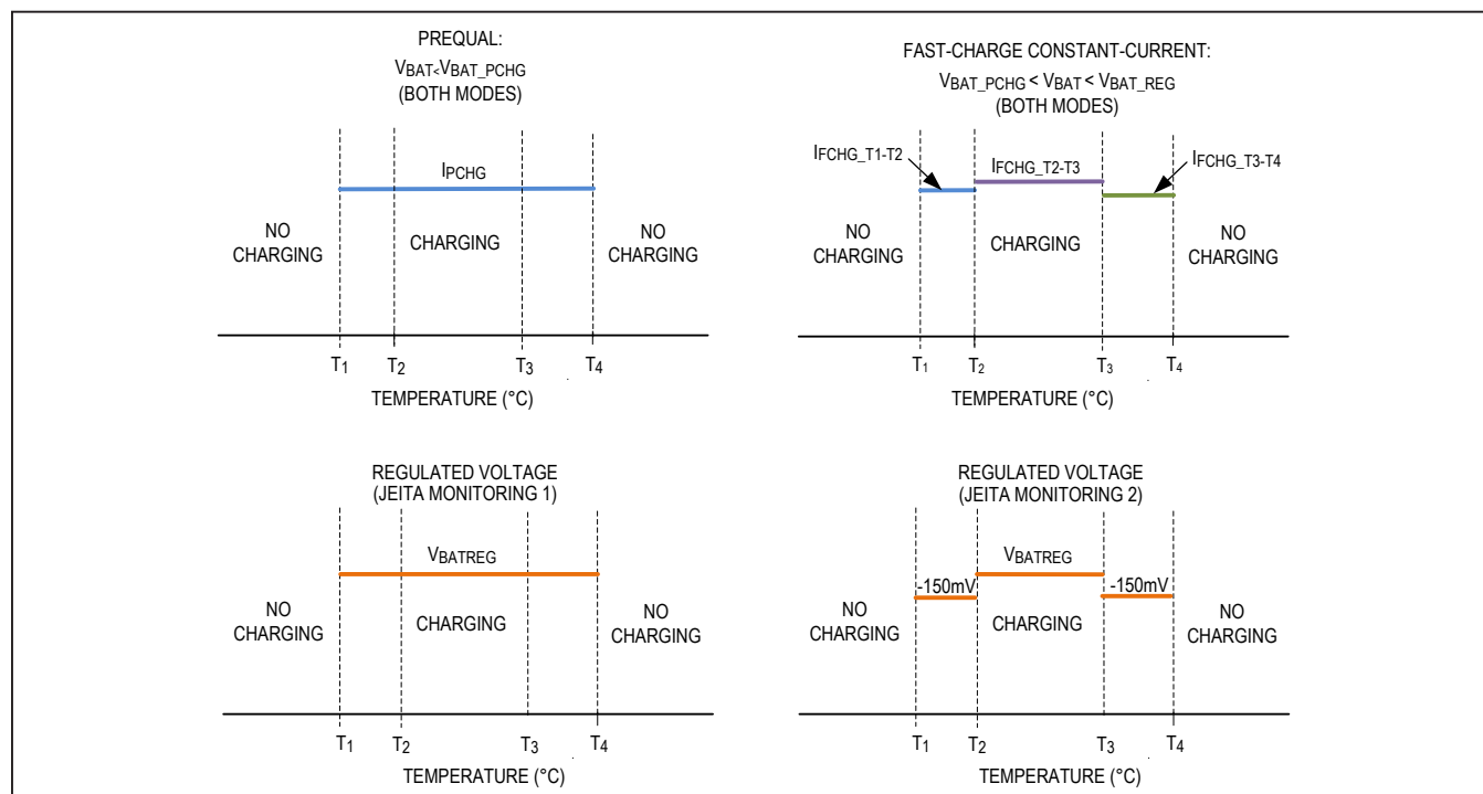
Figure 4b. Charging Behavior Using JEITA Monitoring 1 and 2 Modes
