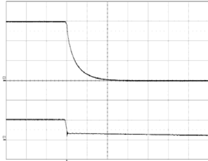
Shut-down enabled by disconnecting V_i at: T_{P1} = +25^{\circ}\text{C} , V_i = 53\text{ V} , I_o = 8\text{ A} resistive load. Top trace: output voltage (5.0 V/div.). Bottom trace: input voltage (50 V/div.). Time scale: (0.5 ms/div.).
