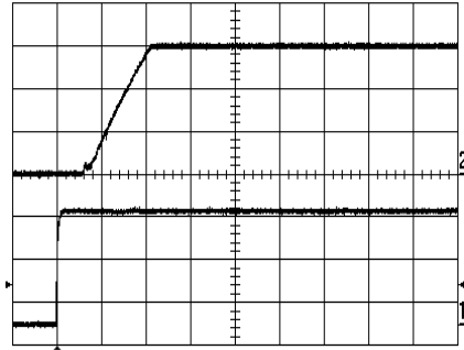
Start-up enabled by connecting V_i at: T_{P1} = +25^{\circ}\text{C} , V_i = 53\text{ V} , I_o = 8\text{ A} resistive load. Top trace: output voltage (5.0 V/div.). Bottom trace: input voltage (20 V/div.). Time scale: (10 ms/div.).
