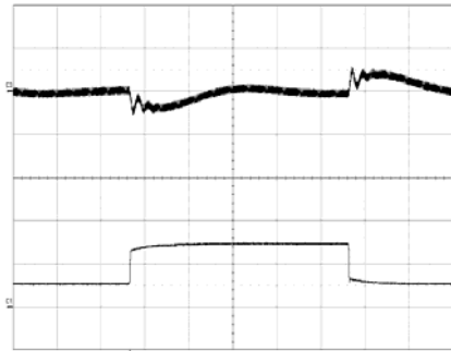
Output voltage response to load current step-change (2-6 A) at: T_{P1} = +25^{\circ}\text{C} , V_i = 53\text{ V} . Top trace: output voltage (500 mV/div.). Bottom trace: load current (4 A/div.). Time scale: (0.1 ms/div.).
