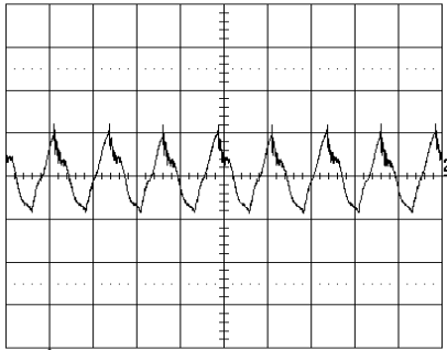
Output voltage ripple at: T_{P1} = +25^{\circ}\text{C} , V_i = 53\text{ V} , I_o = 8\text{ A} resistive load. Trace: output voltage (20 mV/div.). Time scale: (2 μs/div.).
