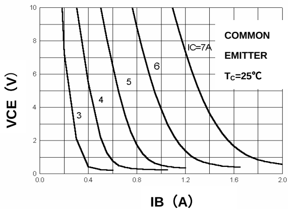
VCE - IB
