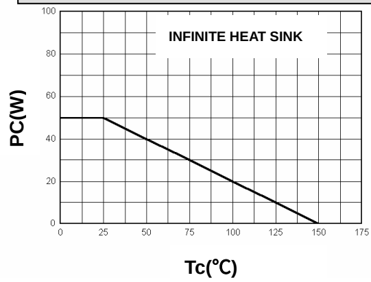
PC-TC
