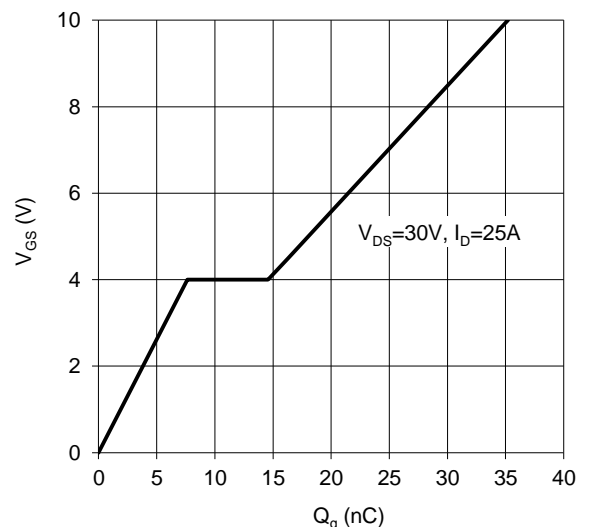
Figure 12. Gate Charge
