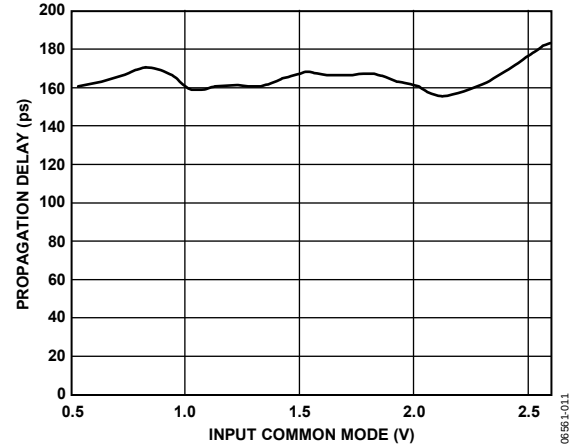
Figure 11. Propagation Delay vs. V_{ICM} ; V_{ID} = 1.6 V p-p
