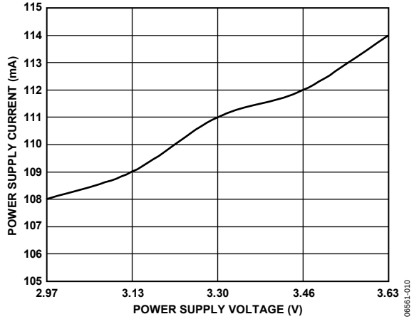
Figure 10. Power Supply Current vs. Power Supply Voltage
