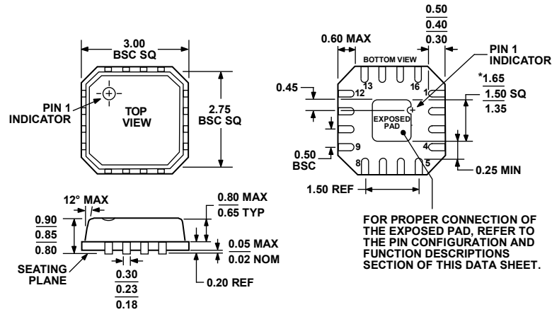
Figure 20. 16-Lead Lead Frame Chip Scale Package [LFCSP_VQ] 3 mm x 3 mm Body, Very Thin Quad (CP-16-3) Dimensions shown in millimeters
