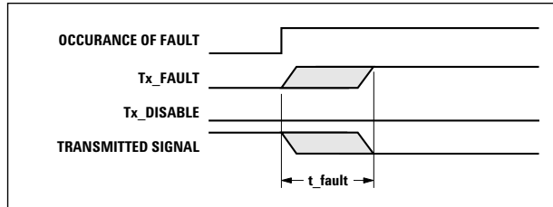
t-fault: TX FAULT ASSERTED, TX SIGNAL NOT RECOVERED
